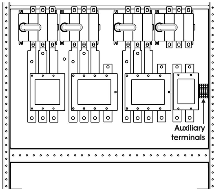
Picture 7 – Position of auxiliary terminals of KEOR HP
