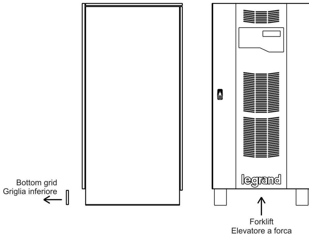
Illustration 2 – Manutention de l'UPS KEOR HP
