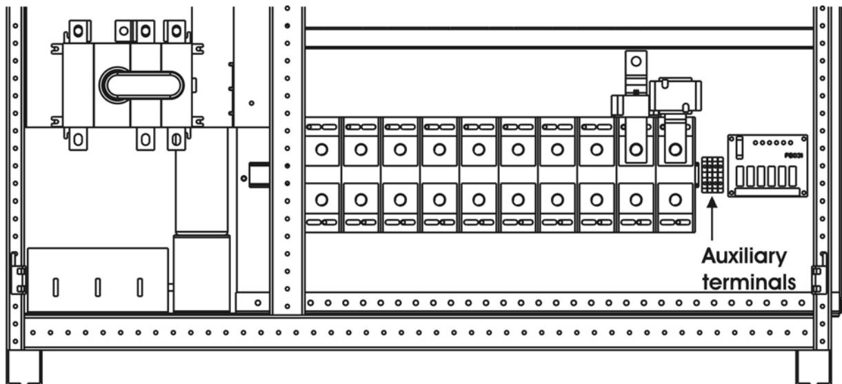
Picture 7 – Position of auxiliary terminals of KEOR HP
