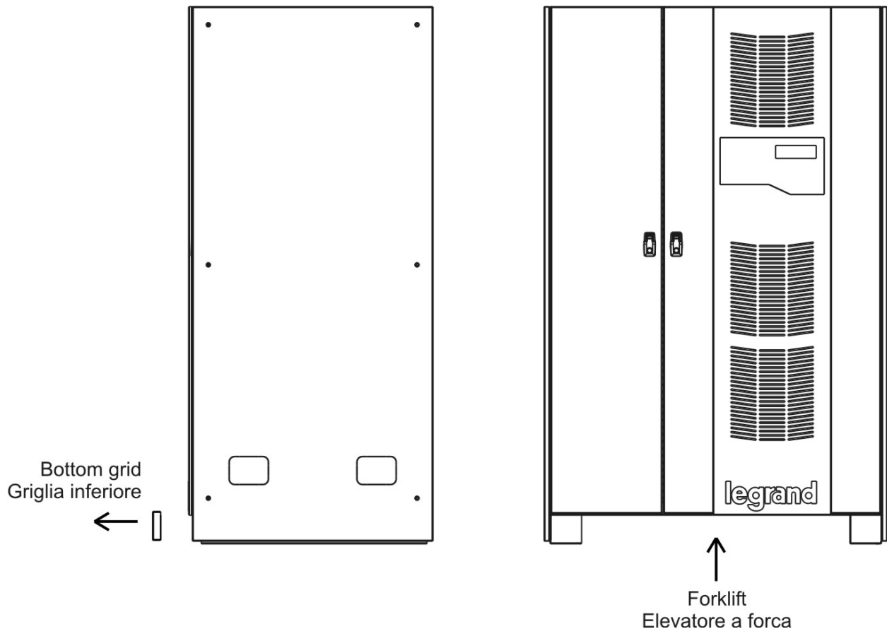
Illustration 2 – Manutention de l'UPS KEOR HP
