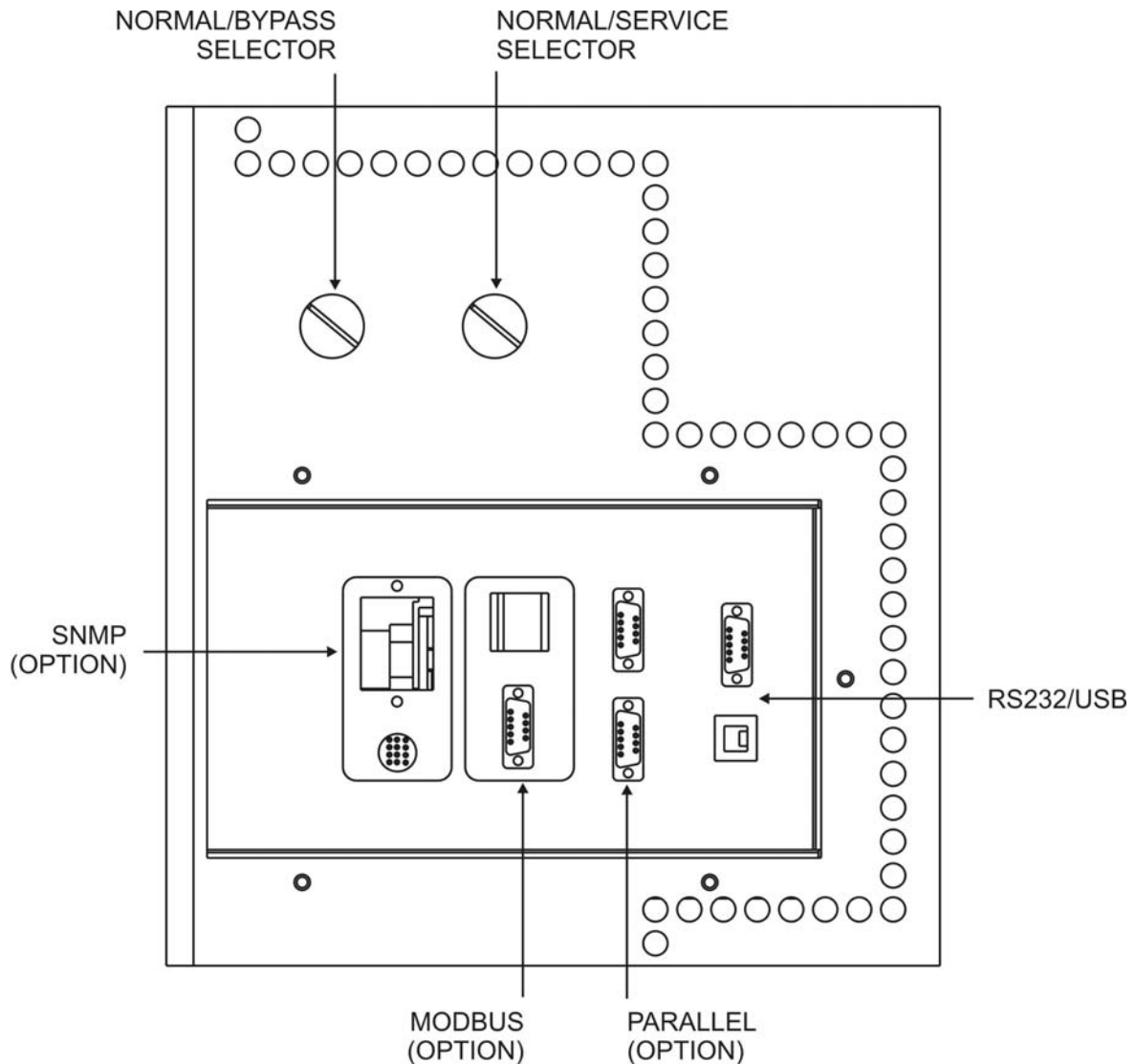
Picture 9 – Interfaces of UPS KEOR HP
