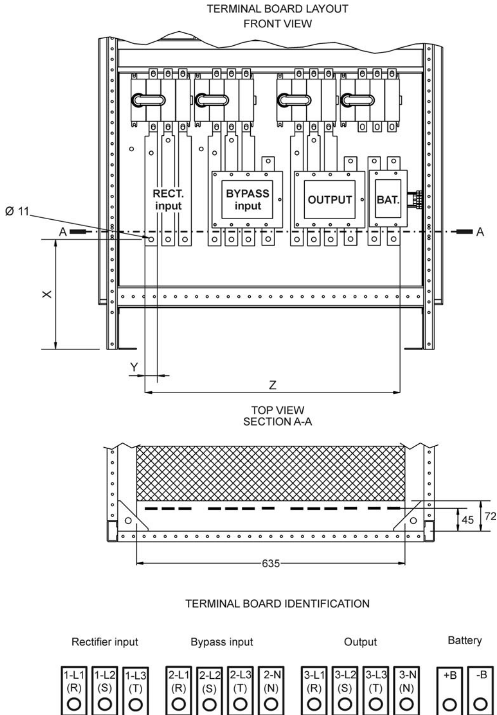
Picture 6 – Position of power terminals of KEOR HP
