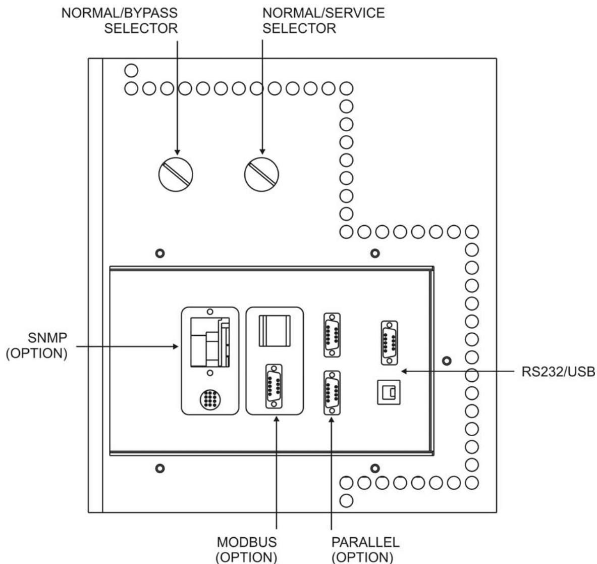
Illustration 9 – Interfaces de l'UPS KEOR HP
