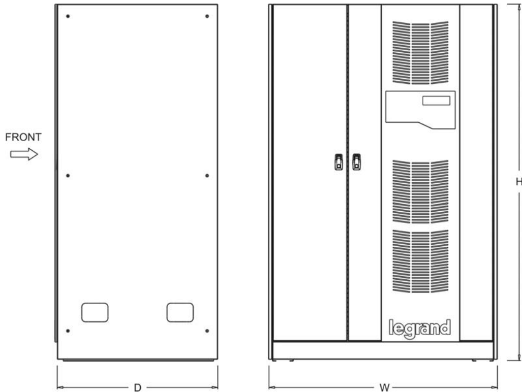
Picture 4 – Overall dimensions of UPS KEOR HP
