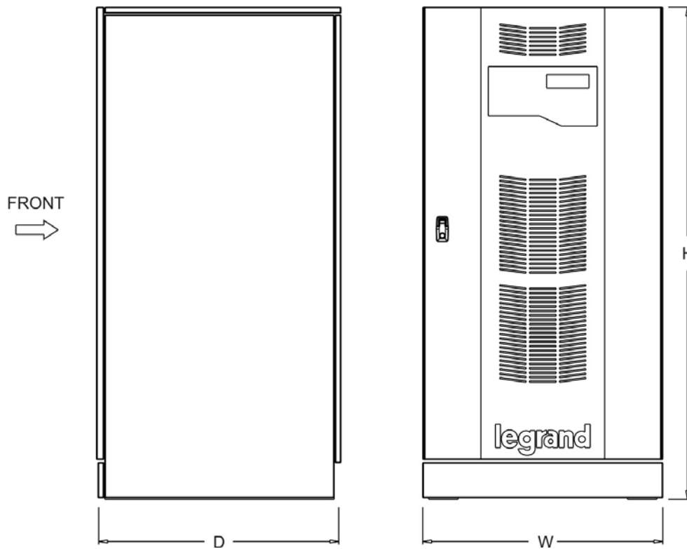
Picture 4 – Overall dimensions of UPS KEOR HP
